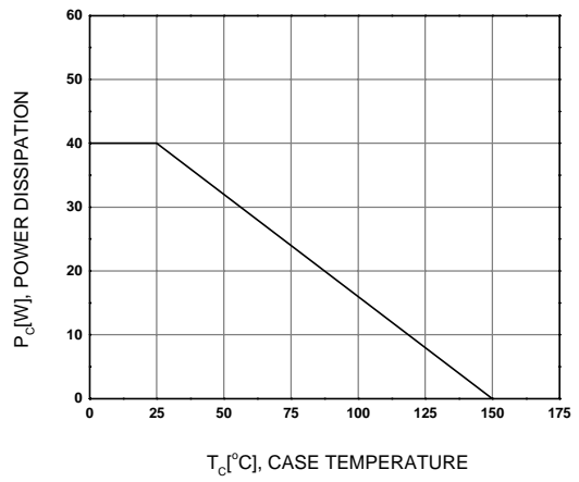
Figure 8. Power Derating
